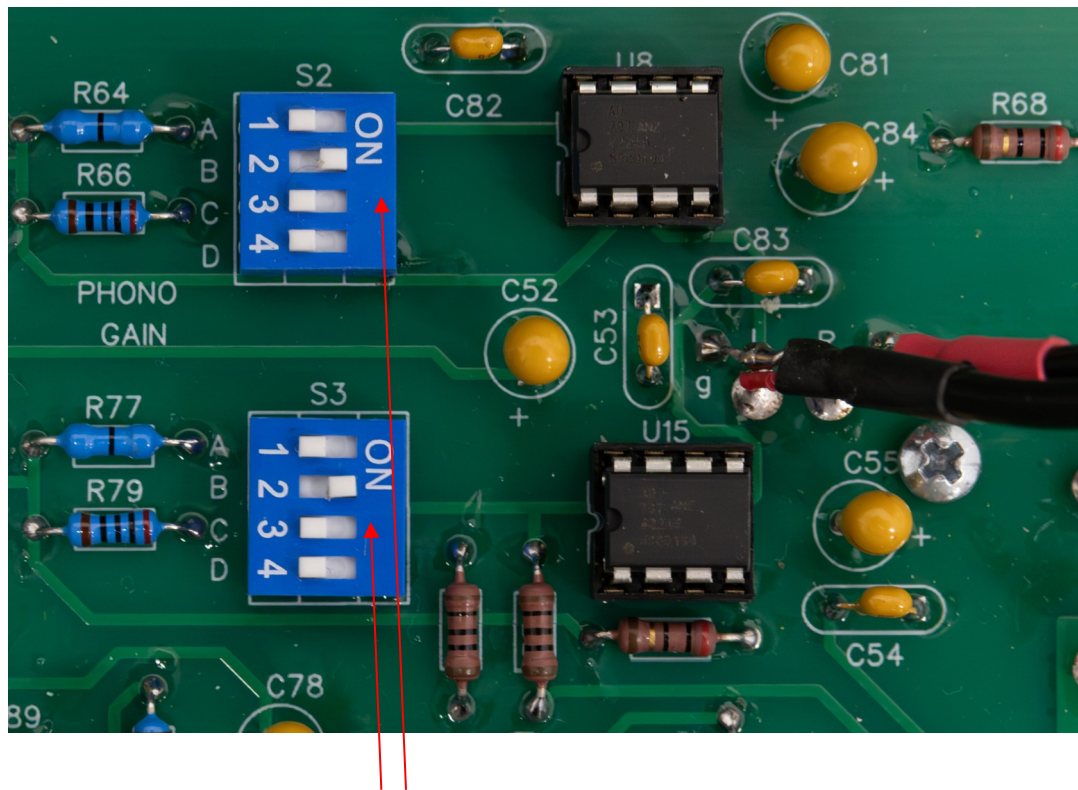
Gain setting DIP switches. Right side towards back of main board.
